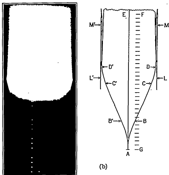
FIGURE 1—An explosion of a mixture of CO, O 2 , and water vapor at constant volume.
