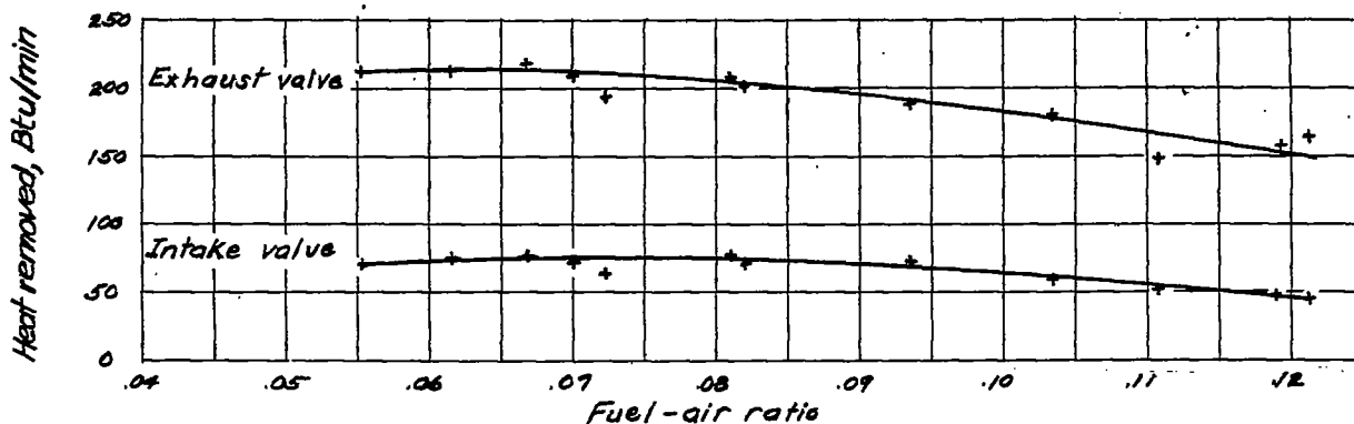
Figure 10.- Heat removed from valves by cooling water at maximum permissible engine output for various fuel-air ratios. Fuel, 100-octane.
