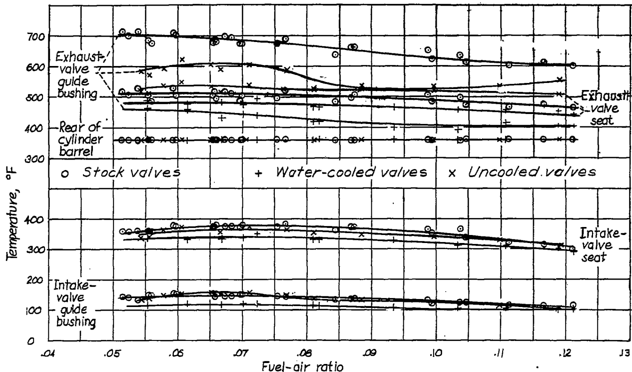
Figure 12. - Valve-seat and valve-guide temperatures at maximum permissible output with various fuel-air ratios. Fuel, 100-octane.
