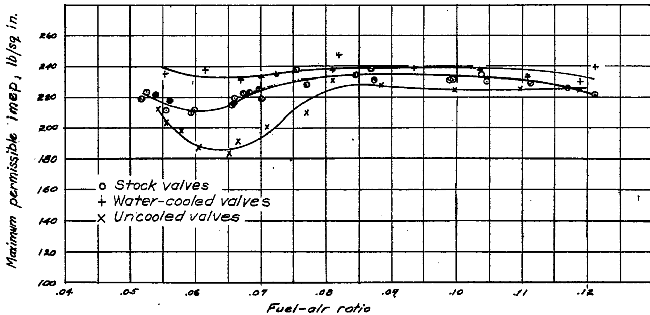
Figure 7 - Comparison of maximum permissible indicated mean effective pressure of various fuel-air ratios. Fuel, 100-octane.
