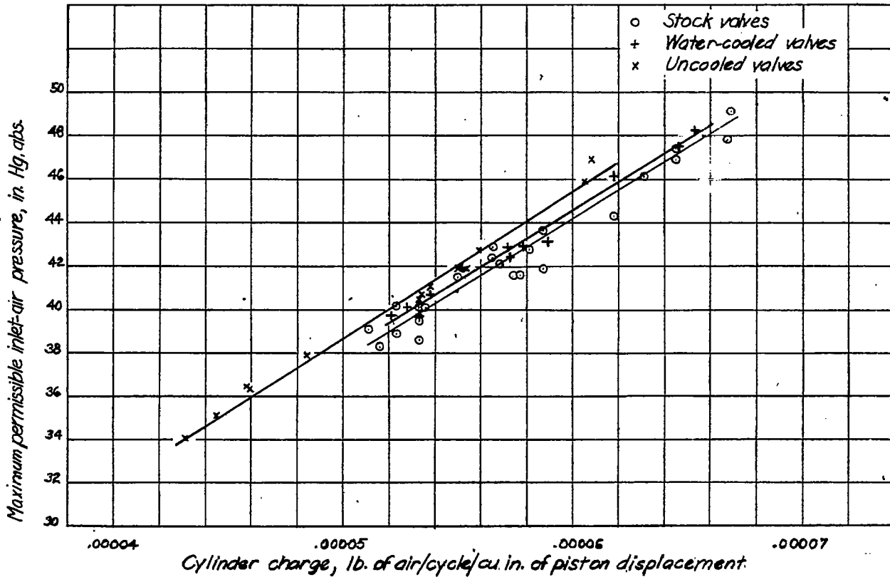
Figure 6.-- Cylinder-charge comparison; stock, water-cooled and uncooled valves. Fuel, 100-octane.
