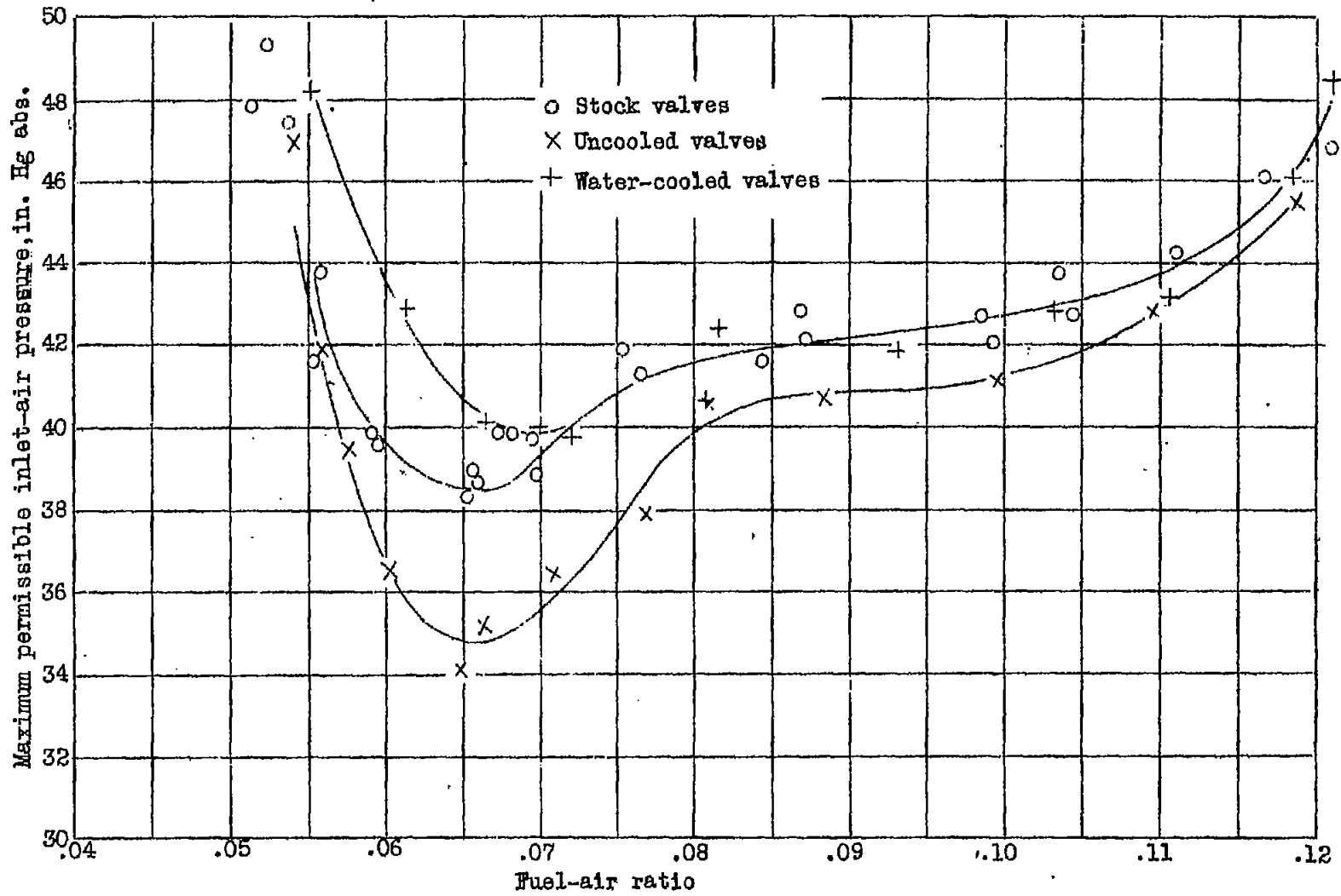
Figure 5.- Comparison of maximum permissible inlet-air pressure at various fuel-air ratios. Fuel, 100-octane.
