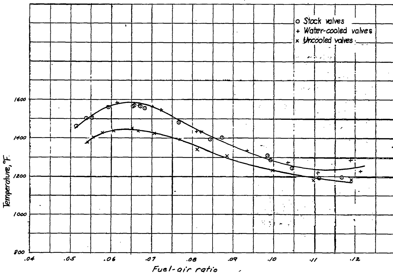
Figure 11. - Exhaust-gas temperature at maximum permissible output with various fuel-air ratios Fuel, 100-octane.
