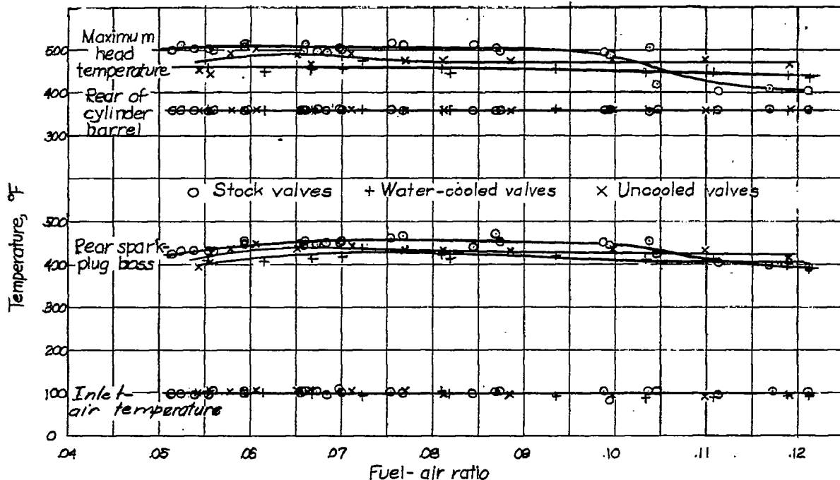
Figure 13. - Temperatures of inlet air and rear spark-plug boss and maximum head temperature at maximum permissible output with various fuel-air ratios. Fuel, 100-octane.
