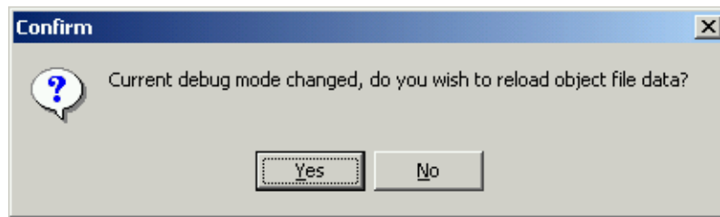
Figure 17. Confirm Window
