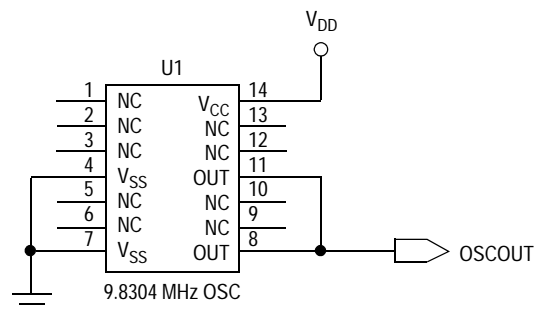
Figure 6a. Canned Oscillator Circuit
