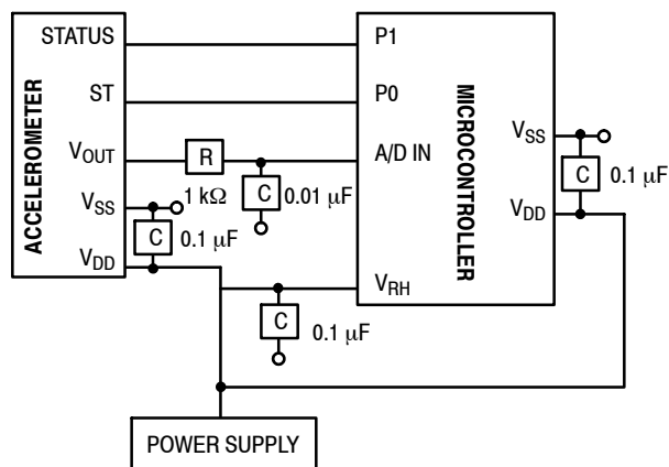
Figure 4. Recommend PCB Layout for Interfacing Accelerometer to Microcontroller
