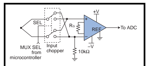
Figure 5—An input chopper like a CD4052 is all that is necessary to null signal conditioner offsets.
