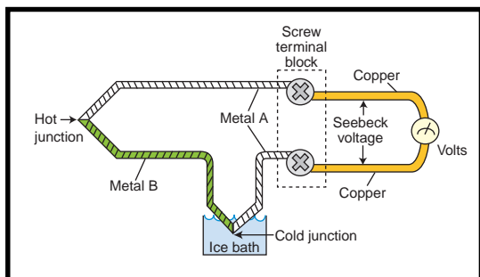
Figure 2 —By inserting a short pigtail of Metal A onto the terminal block where Metal B would normally connect, we move the cold junction.
