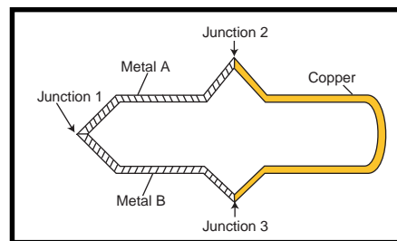
Figure 1c —The act of connecting a measurement system made of copper introduces two parasitic thermocouples.
