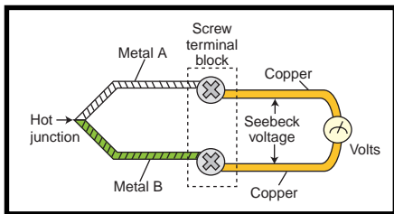
Figure 1b —To use a thermocouple, you must have a measurement system.
