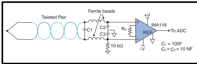
Figure 4—The common-mode filter and common-mode rejection characteristics pay off in thermocouple amplifiers.
