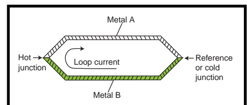
Figure 1a—Two wires are all that are required to form a thermocouple.
