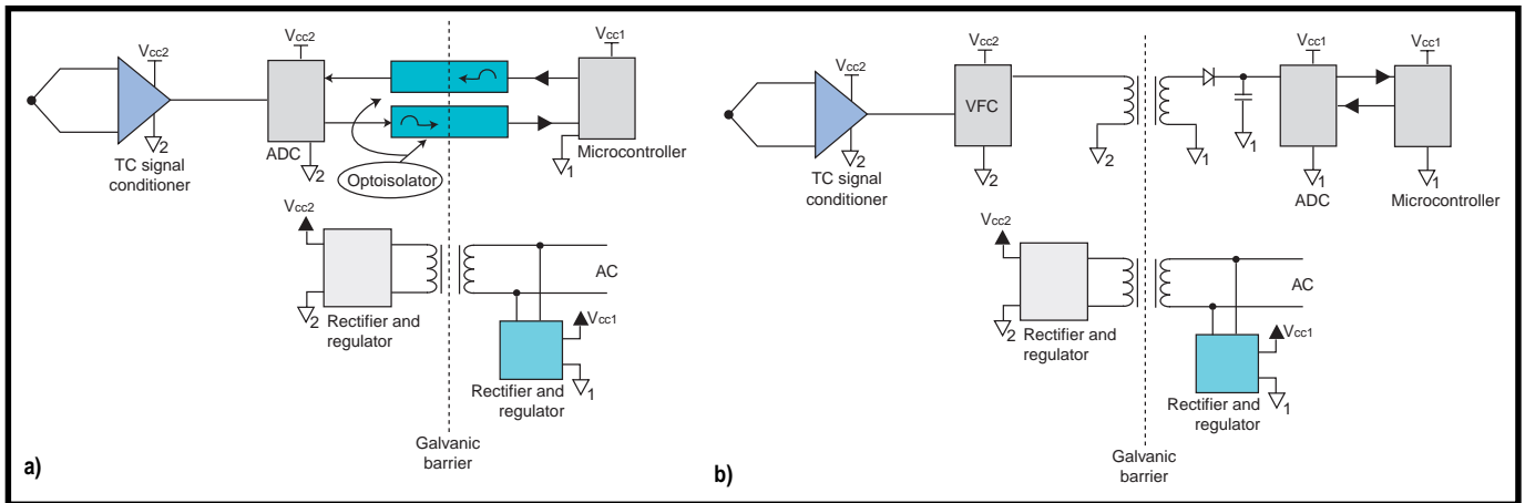
Figure 3 —Galvanic isolation to a few thousand volts is easy (but a little expensive) using opto-isolation (a) and inexpensive (but a bit more challenging) using a VFC and a transformer (b).
